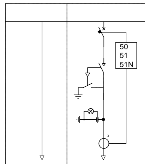
SCHEMA UNIFILARE QUADRO WTG OS_04 E OS_01
