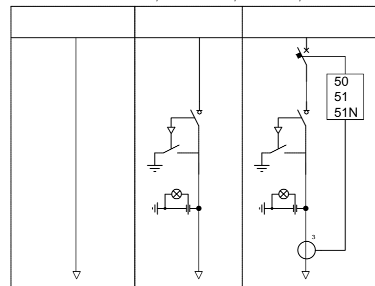
SCHEMA UNIFILARE QUADRO WTG OS_02, OS_03, OS_05, OS_06
